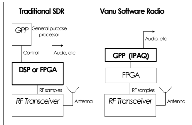
Figure 1: A comparison of the traditional software defined radio architecture and the Vanu Software Radio architecture
